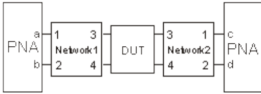
Topology C
