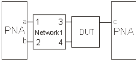
Topology B
